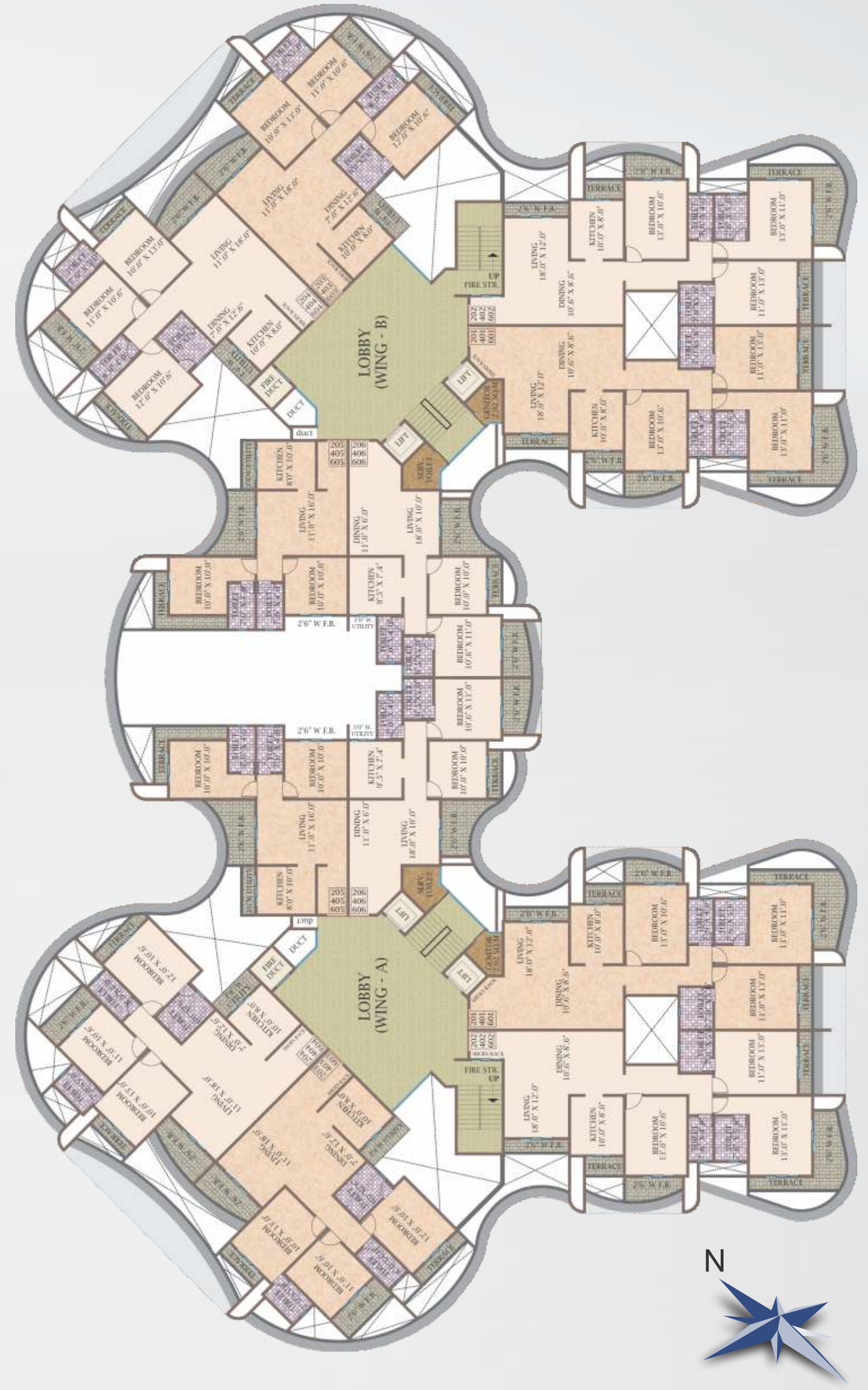
TYPICAL - 2nd, 4th, 6th - FLOOR PLAN
