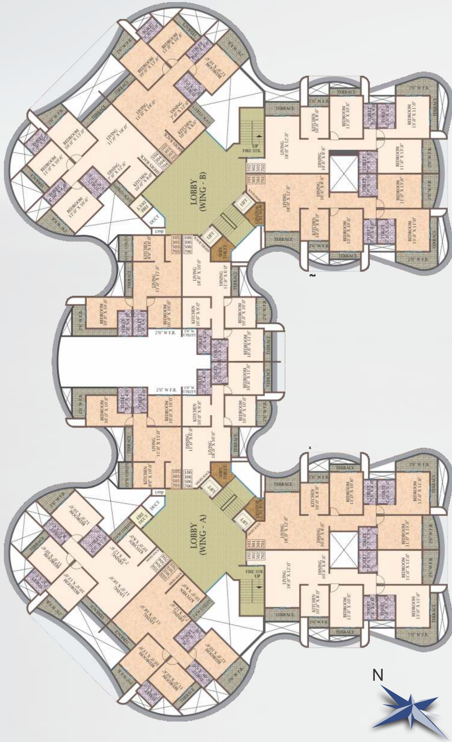
TYPICAL - 1st, 3rd, 5th, 7th - FLOOR PLAN
